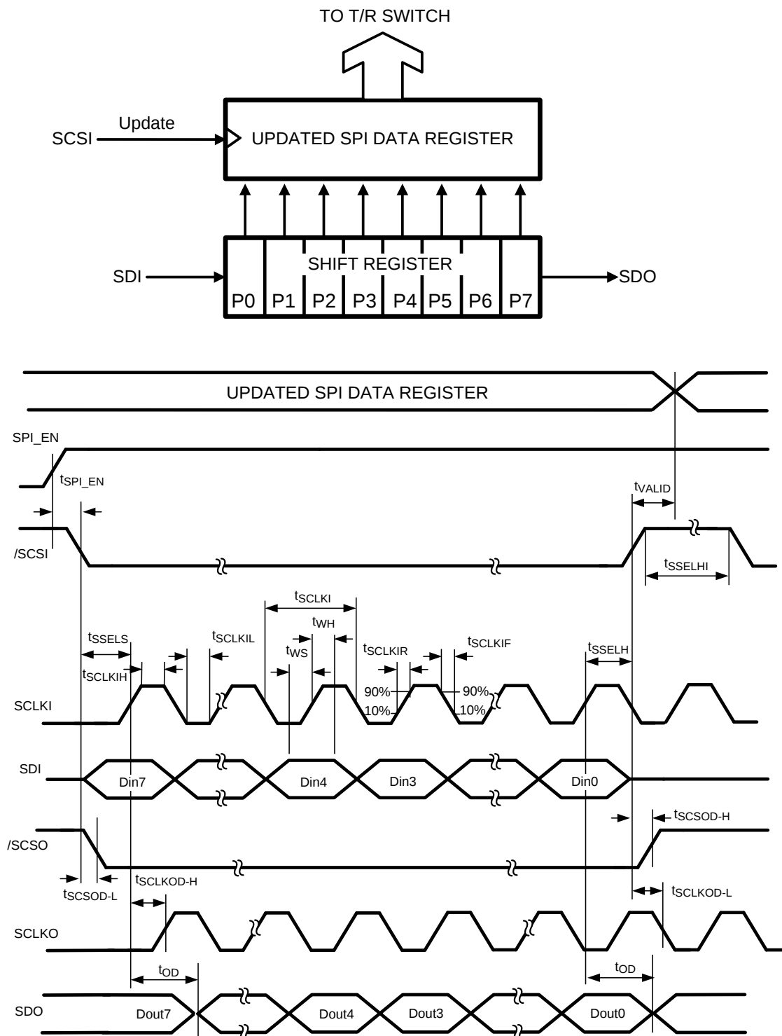
Figure 4. SPI™ Timing Diagram
